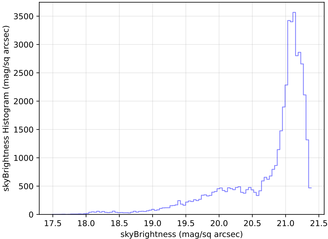
noroll_mjdp180_v3.4_10yrs Yr 1 r band: skyBrightness Histogram
