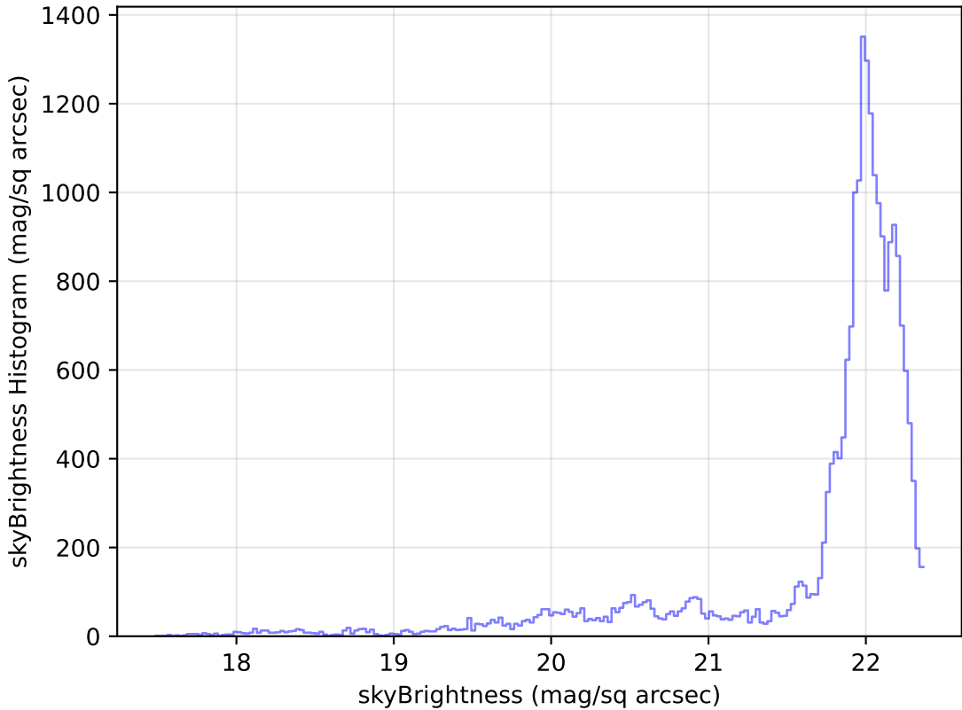
noroll_mjdp180_v3.4_10yrs Yr 1 g band: skyBrightness Histogram
