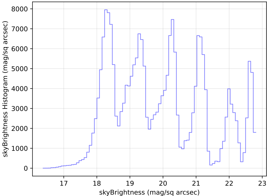
noroll_mjdp180_v3.4_10yrs Yr 1 all bands: skyBrightness Histogram
