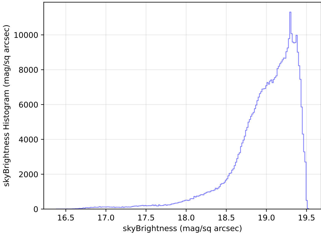
noroll_mjdp180_v3.4_10yrs WFD z band: skyBrightness Histogram
