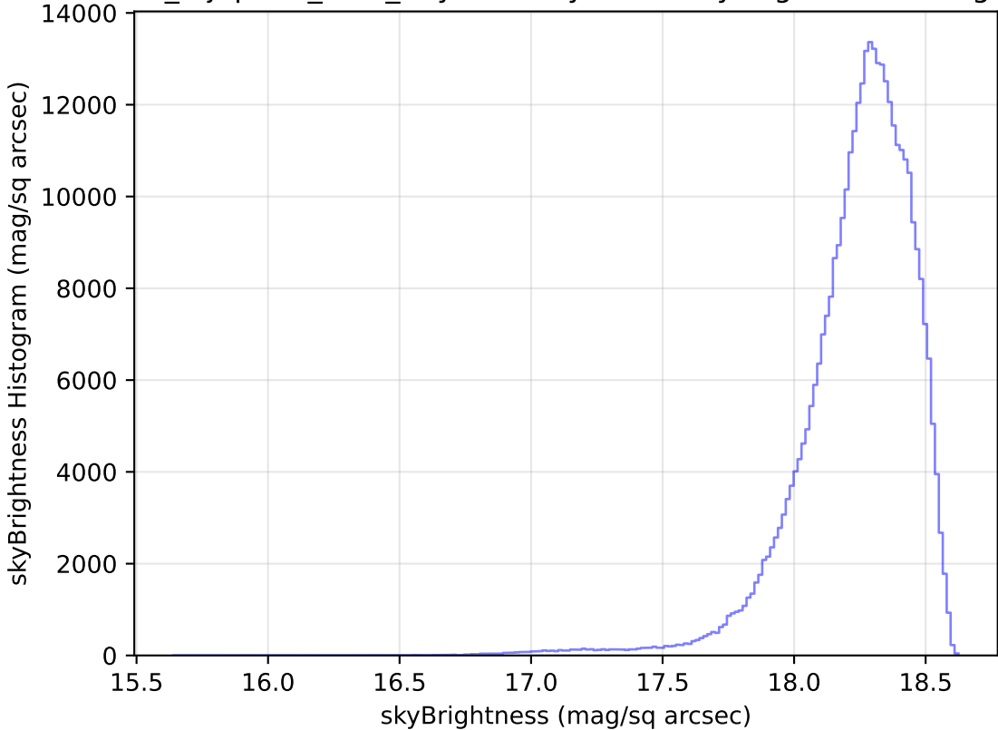
noroll_mjdp180_v3.4_10yrs WFD y band: skyBrightness Histogram
