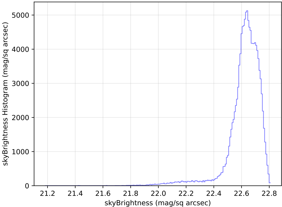
noroll_mjdp180_v3.4_10yrs WFD u band: skyBrightness Histogram
