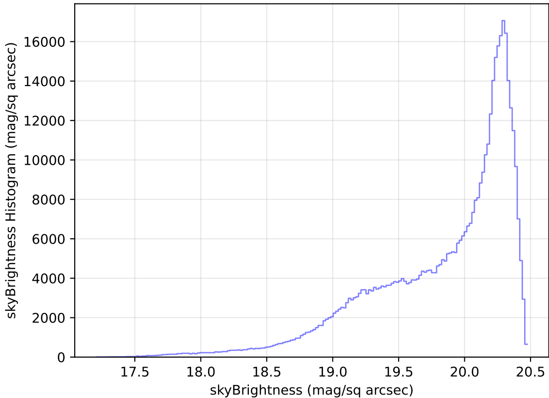
noroll_mjdp180_v3.4_10yrs WFD i band: skyBrightness Histogram
