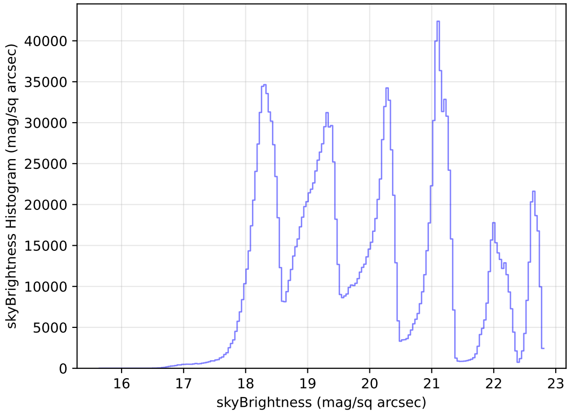
noroll_mjdp180_v3.4_10yrs WFD all bands: skyBrightness Histogram
