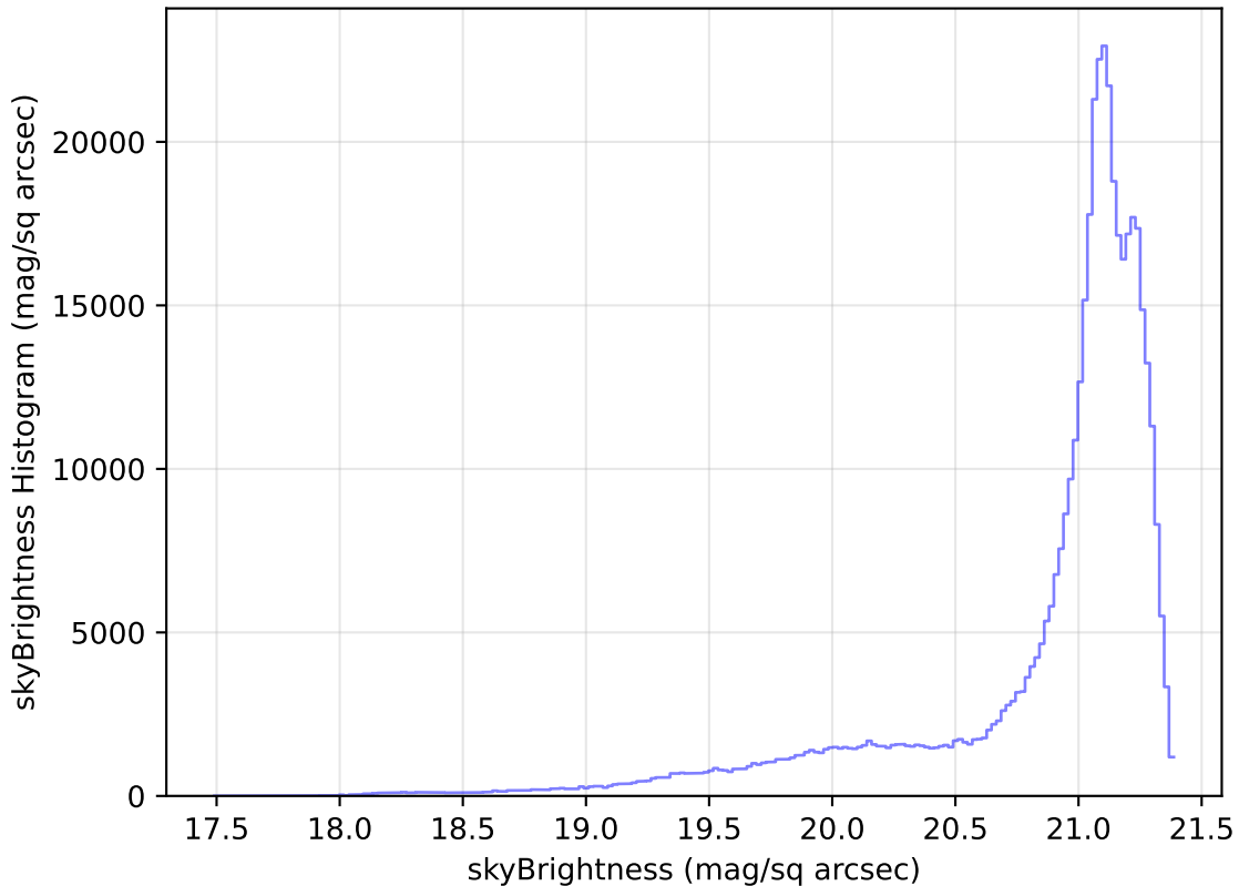
noroll_mjdp180_v3.4_10yrs All sky r band: skyBrightness Histogram
