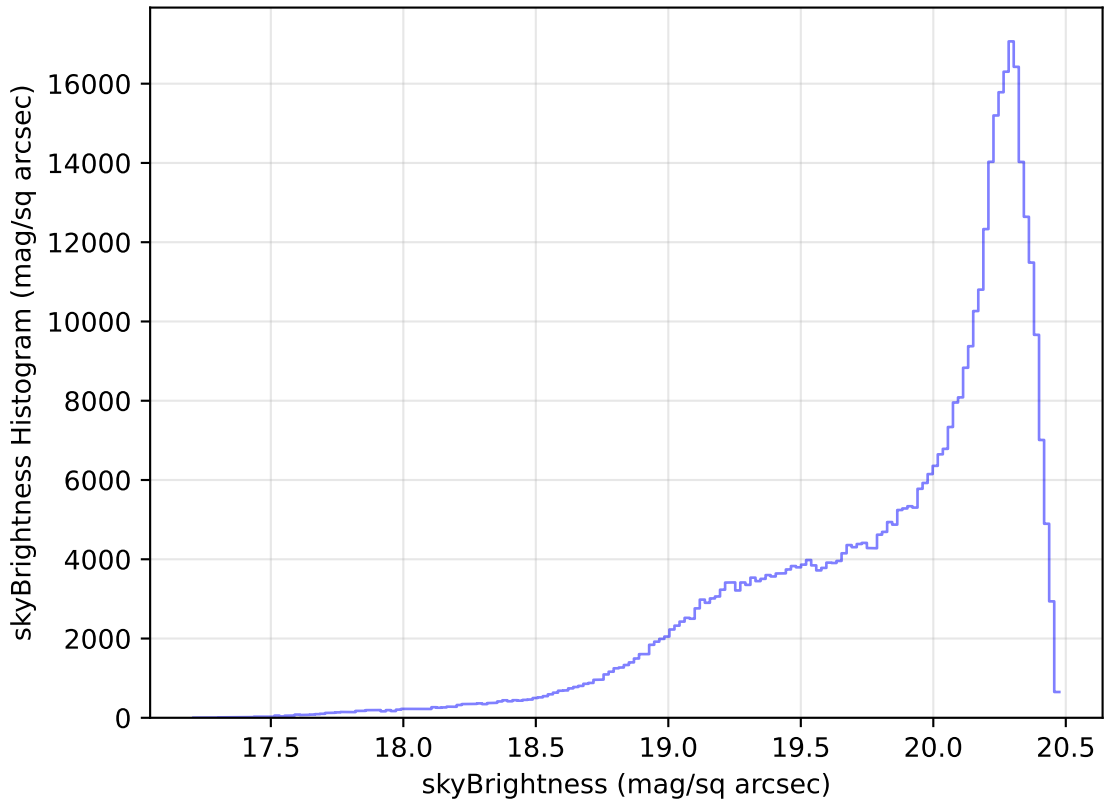
noroll_mjdp180_v3.4_10yrs All sky i band: skyBrightness Histogram
