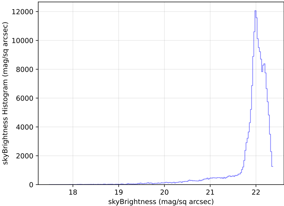
noroll_mjdp180_v3.4_10yrs All sky g band: skyBrightness Histogram
