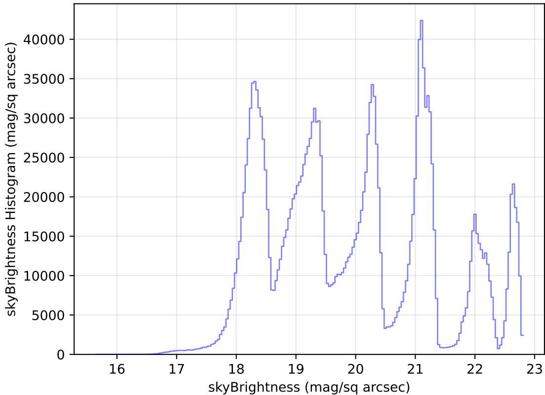
noroll_mjdp180_v3.4_10yrs All sky all bands: skyBrightness Histogram
