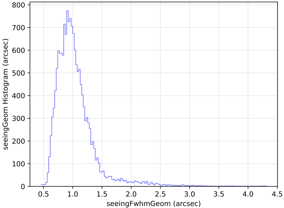
noroll_mjdp180_v3.4_10yrs Yr 1 u band: seeingGeom Histogram
