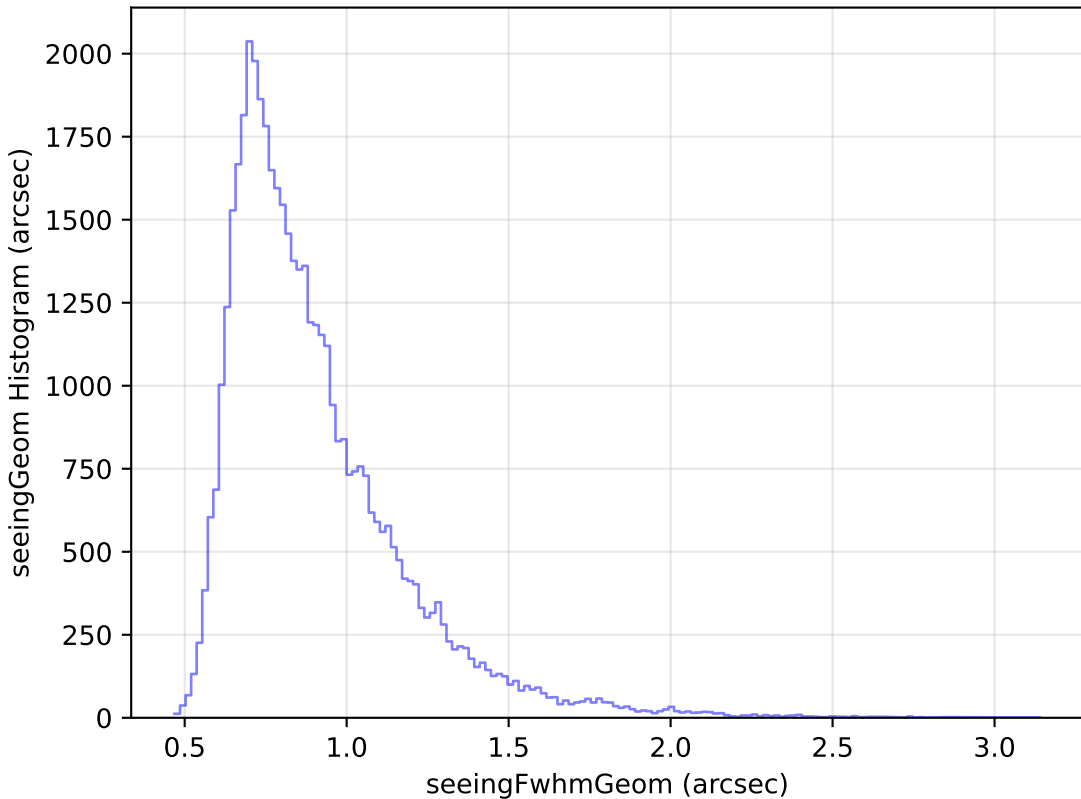
noroll_mjdp180_v3.4_10yrs Yr 1 r band: seeingGeom Histogram
