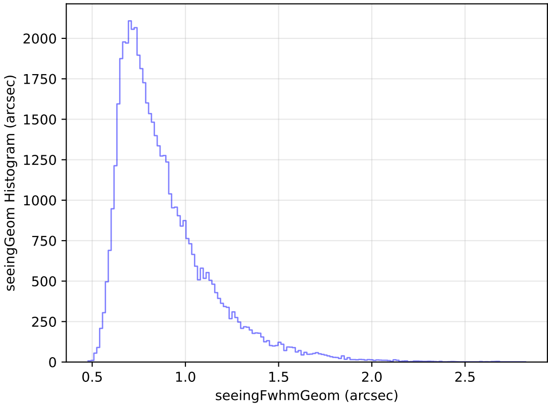
noroll_mjdp180_v3.4_10yrs Yr 1 i band: seeingGeom Histogram
