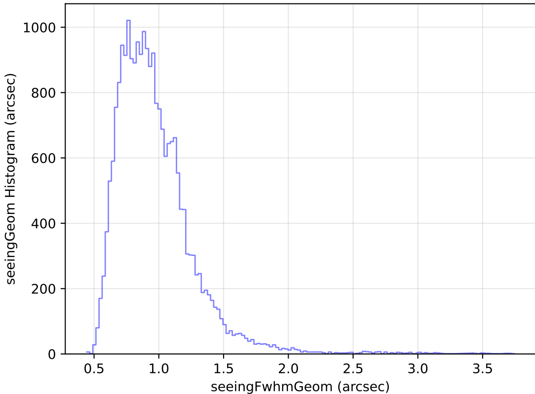
noroll_mjdp180_v3.4_10yrs Yr 1 g band: seeingGeom Histogram
