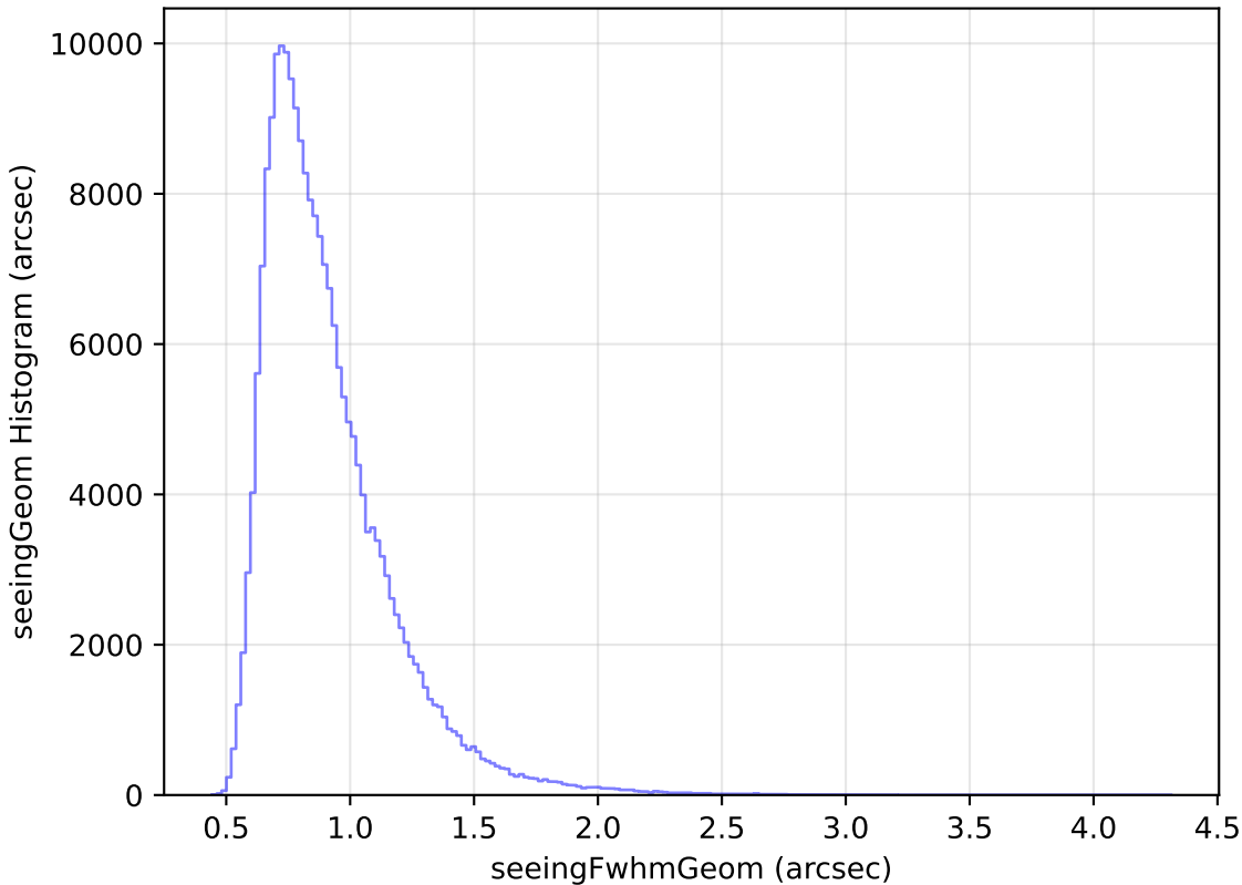
noroll_mjdp180_v3.4_10yrs Yr 1 all bands: seeingGeom Histogram
