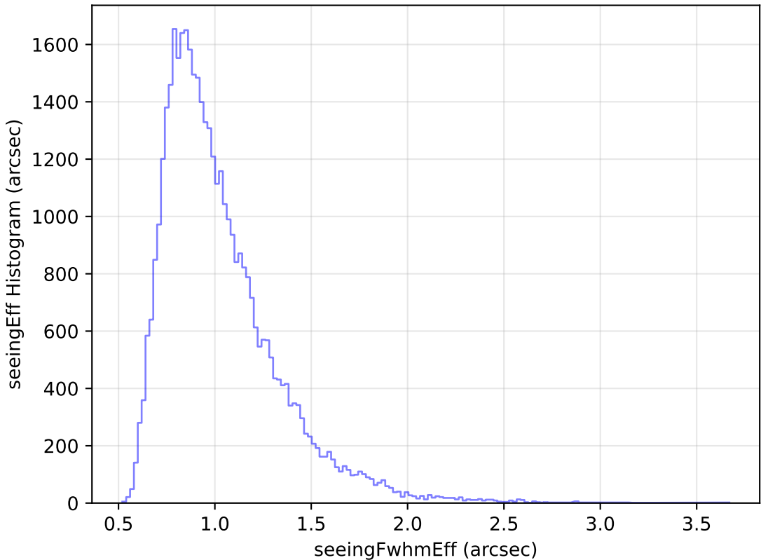
noroll_mjdp180_v3.4_10yrs Yr 1 z band: seeingEff Histogram
