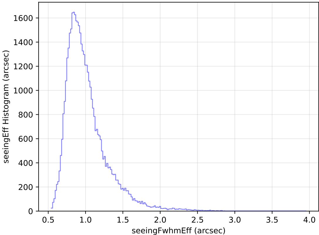
noroll_mjdp180_v3.4_10yrs Yr 1 y band: seeingEff Histogram
