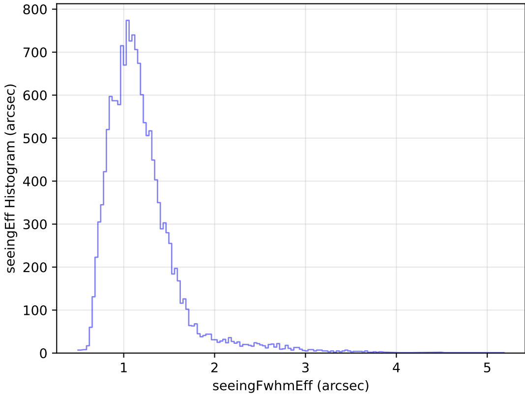
noroll_mjdp180_v3.4_10yrs Yr 1 u band: seeingEff Histogram
