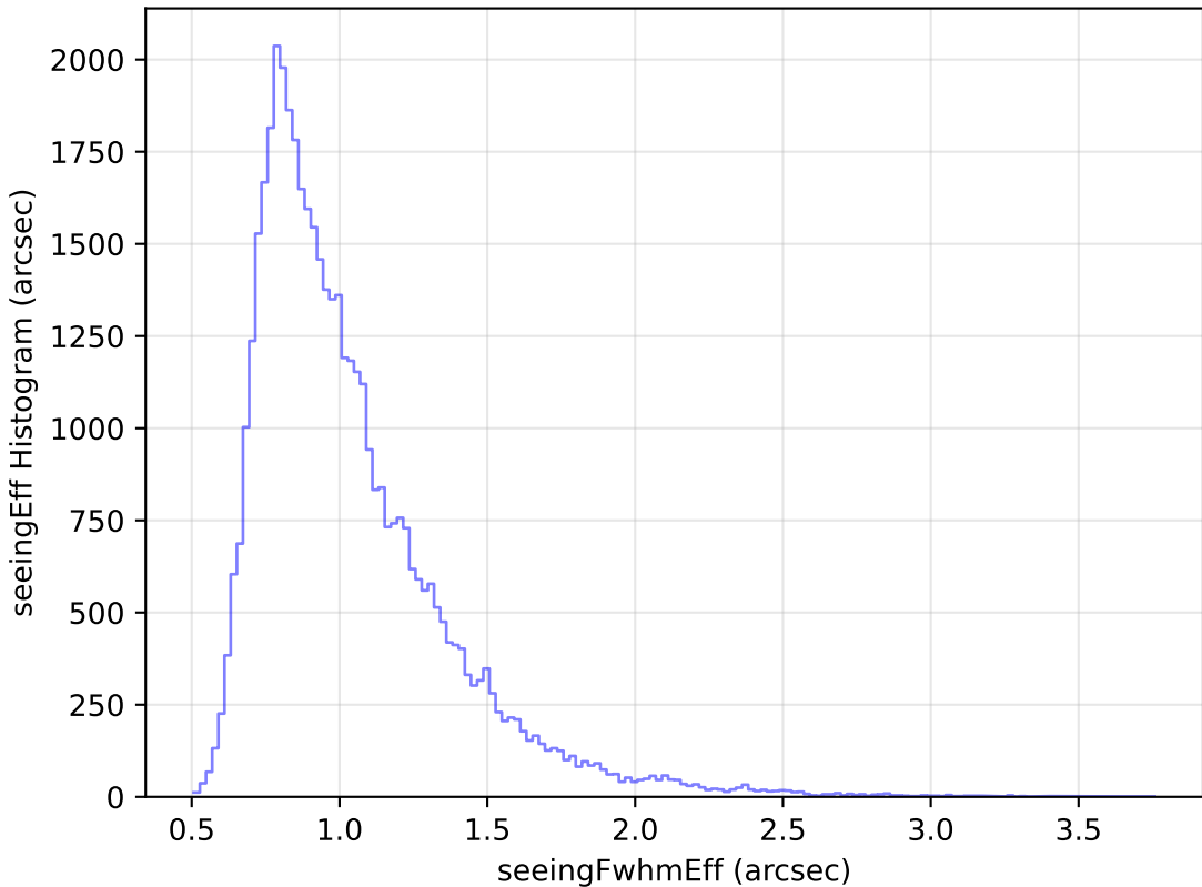
noroll_mjdp180_v3.4_10yrs Yr 1 r band: seeingEff Histogram
