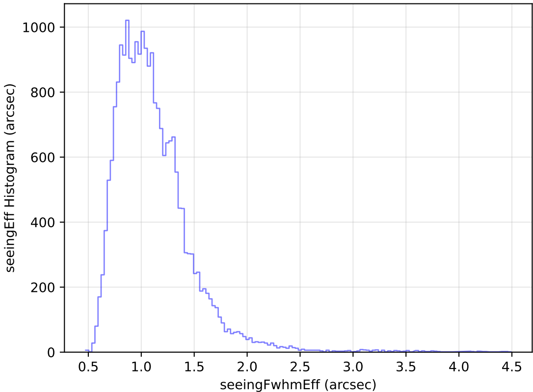
noroll_mjdp180_v3.4_10yrs Yr 1 g band: seeingEff Histogram
