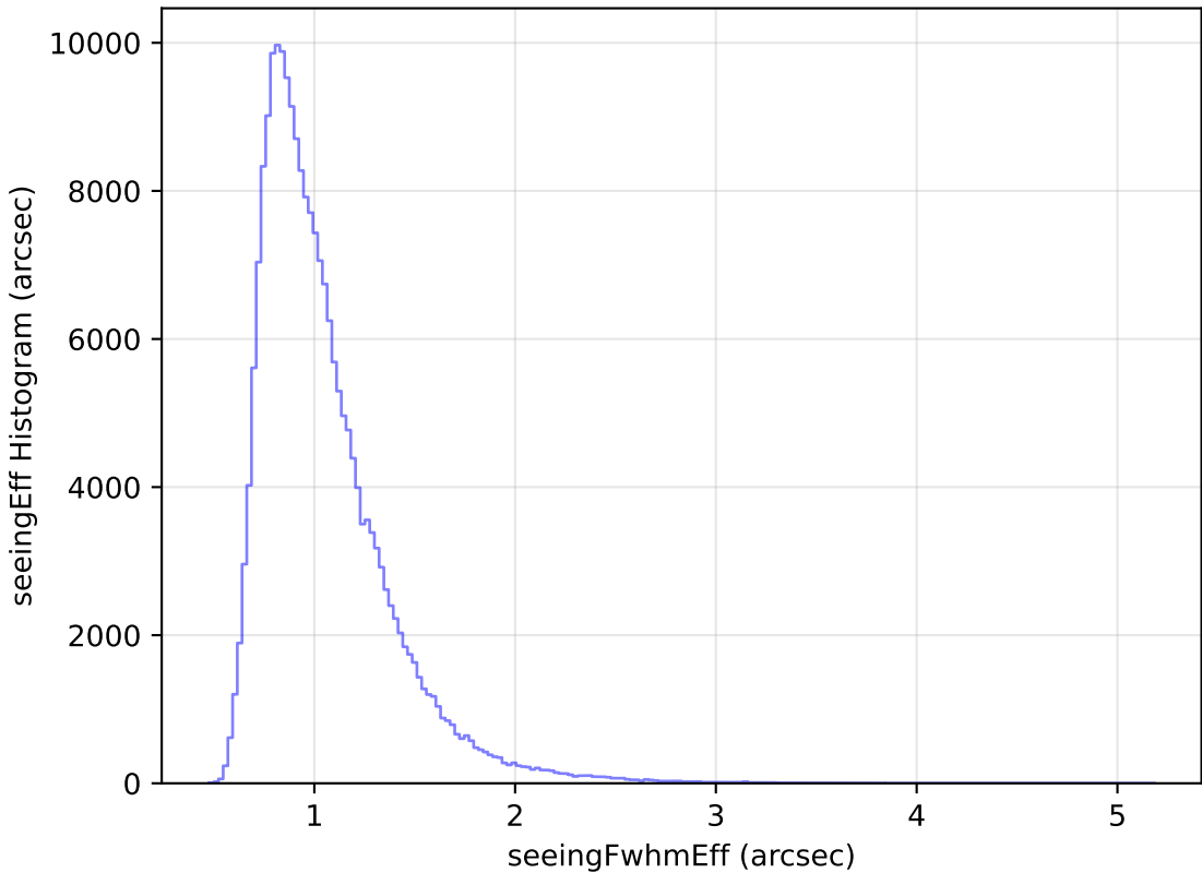
noroll_mjdp180_v3.4_10yrs Yr 1 all bands: seeingEff Histogram
