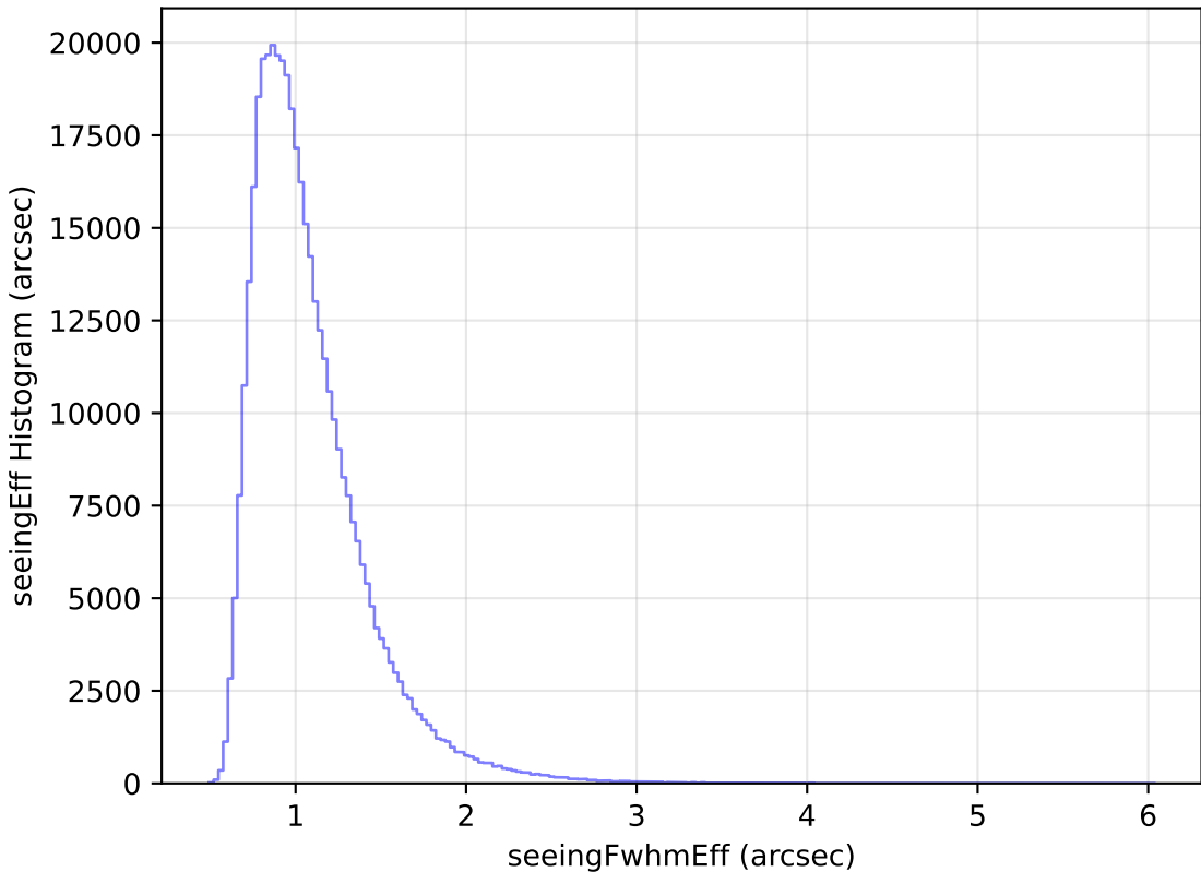
noroll_mjdp180_v3.4_10yrs WFD z band: seeingEff Histogram
