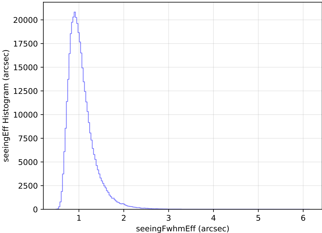
noroll_mjdp180_v3.4_10yrs WFD y band: seeingEff Histogram
