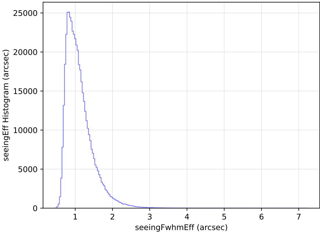
noroll_mjdp180_v3.4_10yrs WFD r band: seeingEff Histogram
