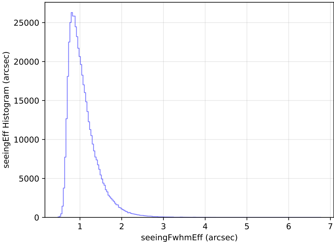
noroll_mjdp180_v3.4_10yrs WFD i band: seeingEff Histogram
