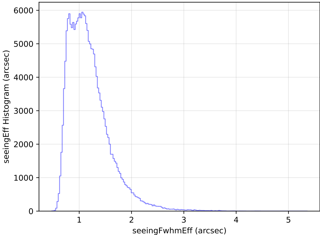
noroll_mjdp180_v3.4_10yrs WFD g band: seeingEff Histogram
