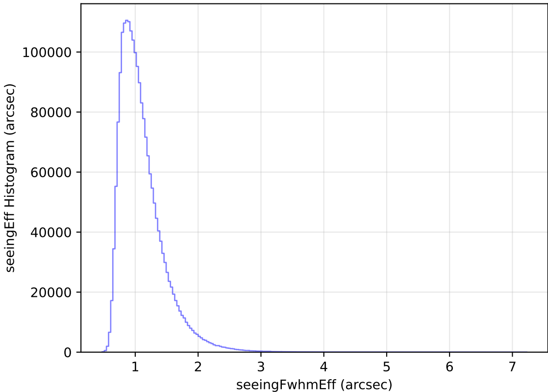
noroll_mjdp180_v3.4_10yrs WFD all bands: seeingEff Histogram
