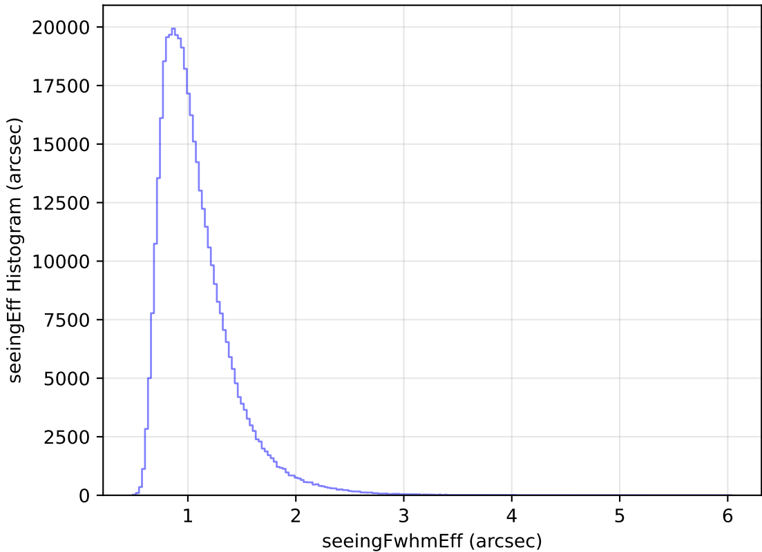
noroll_mjdp180_v3.4_10yrs All sky z band: seeingEff Histogram
