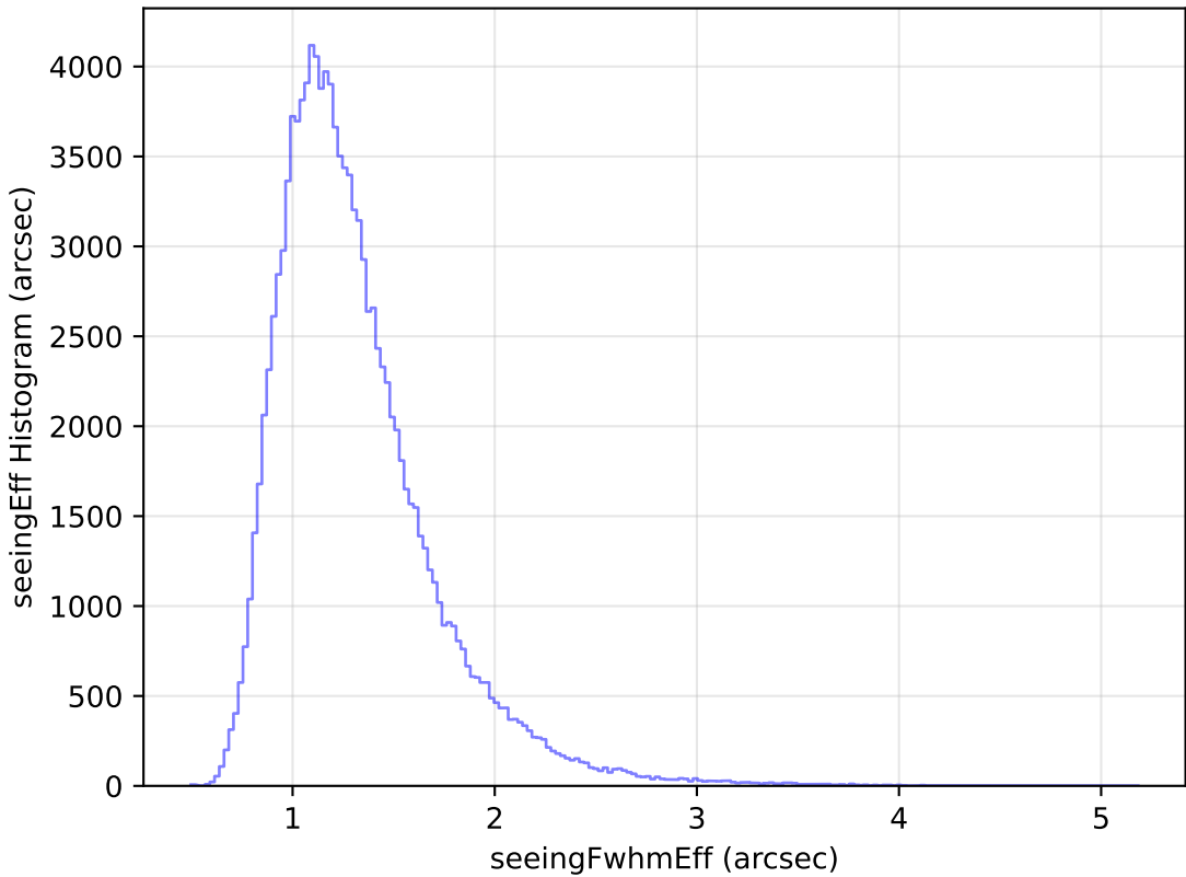
noroll_mjdp180_v3.4_10yrs All sky u band: seeingEff Histogram
