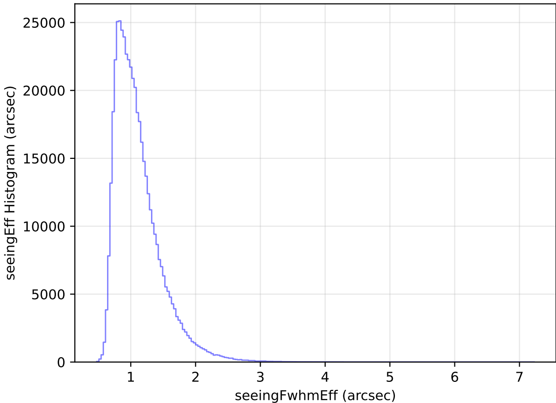
noroll_mjdp180_v3.4_10yrs All sky r band: seeingEff Histogram
