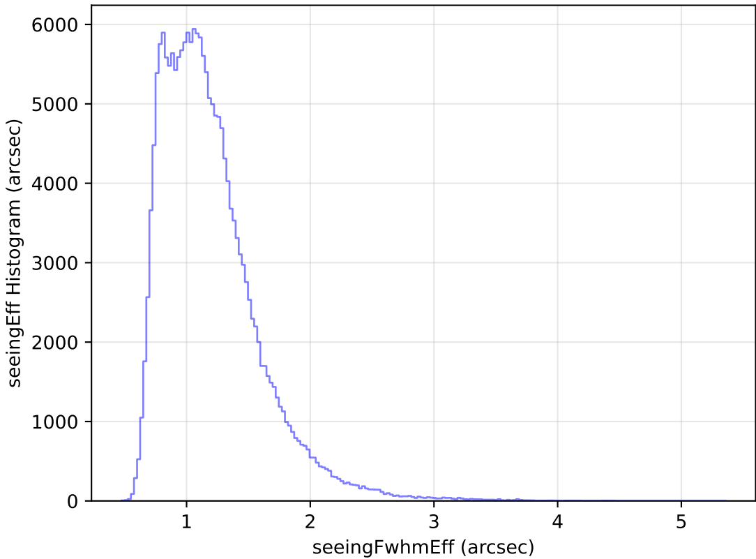
noroll_mjdp180_v3.4_10yrs All sky g band: seeingEff Histogram
