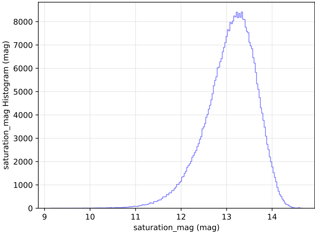
noroll_mjdp180_v3.4_10yrs WFD y band: saturation_mag Histogram
