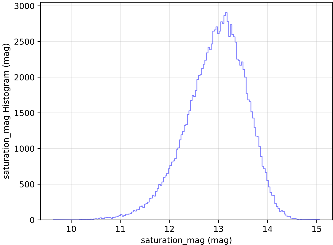
noroll_mjdp180_v3.4_10yrs WFD u band: saturation_mag Histogram
