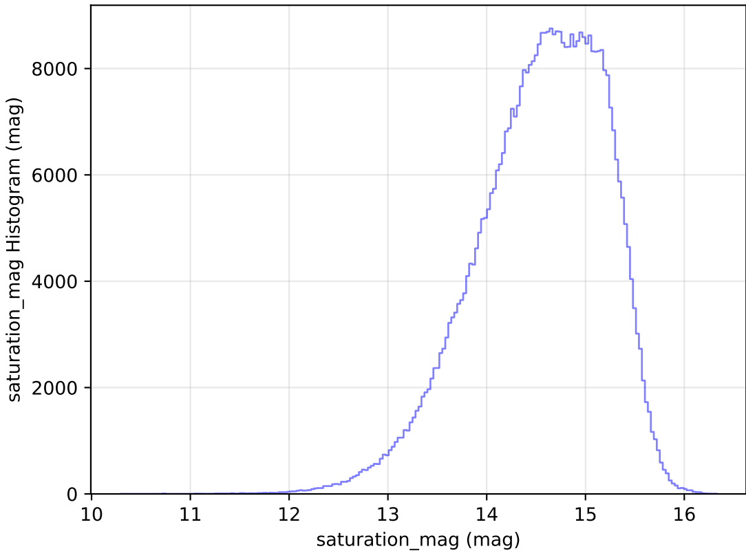
noroll_mjdp180_v3.4_10yrs WFD r band: saturation_mag Histogram
