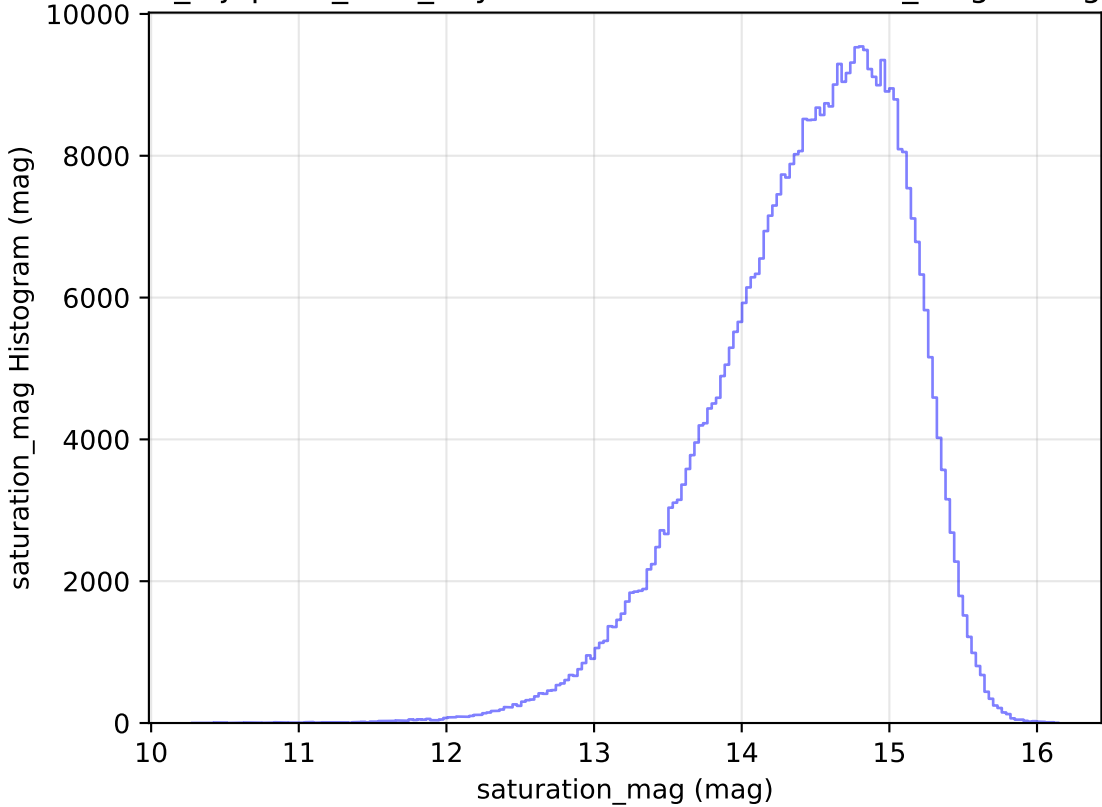
noroll_mjdp180_v3.4_10yrs WFD i band: saturation_mag Histogram
