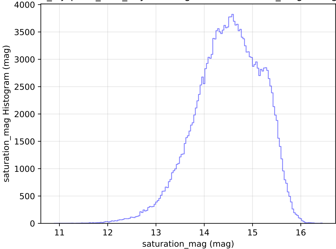
noroll_mjdp180_v3.4_10yrs WFD g band: saturation_mag Histogram
