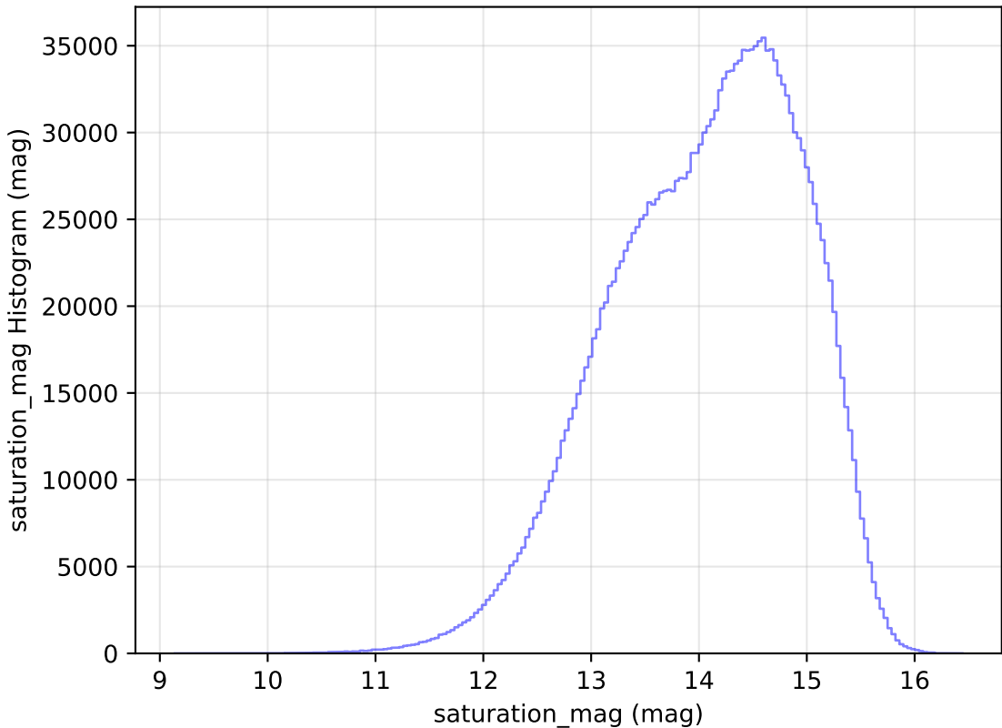
noroll_mjdp180_v3.4_10yrs WFD all bands: saturation_mag Histogram
