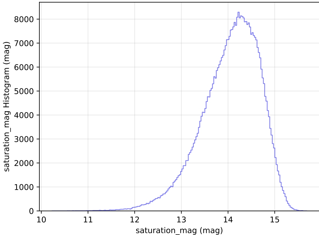
noroll_mjdp180_v3.4_10yrs All sky z band: saturation_mag Histogram
