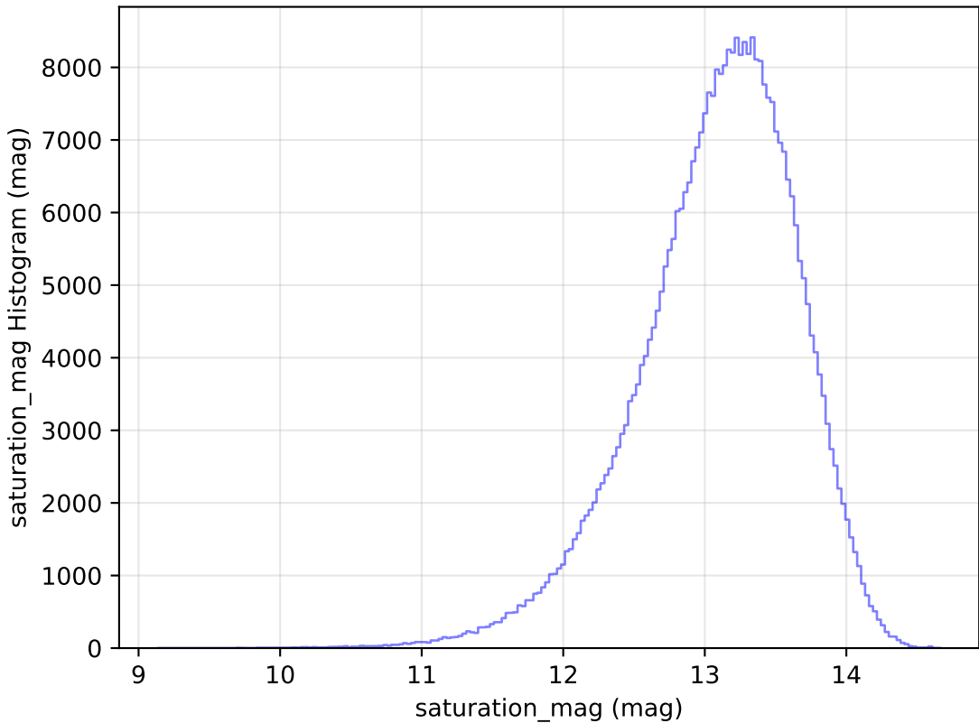
noroll_mjdp180_v3.4_10yrs All sky y band: saturation_mag Histogram
