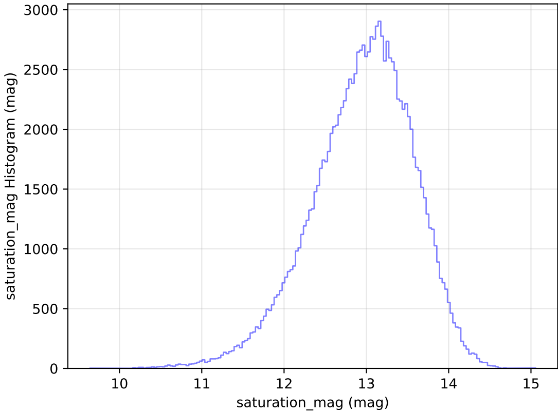
noroll_mjdp180_v3.4_10yrs All sky u band: saturation_mag Histogram
