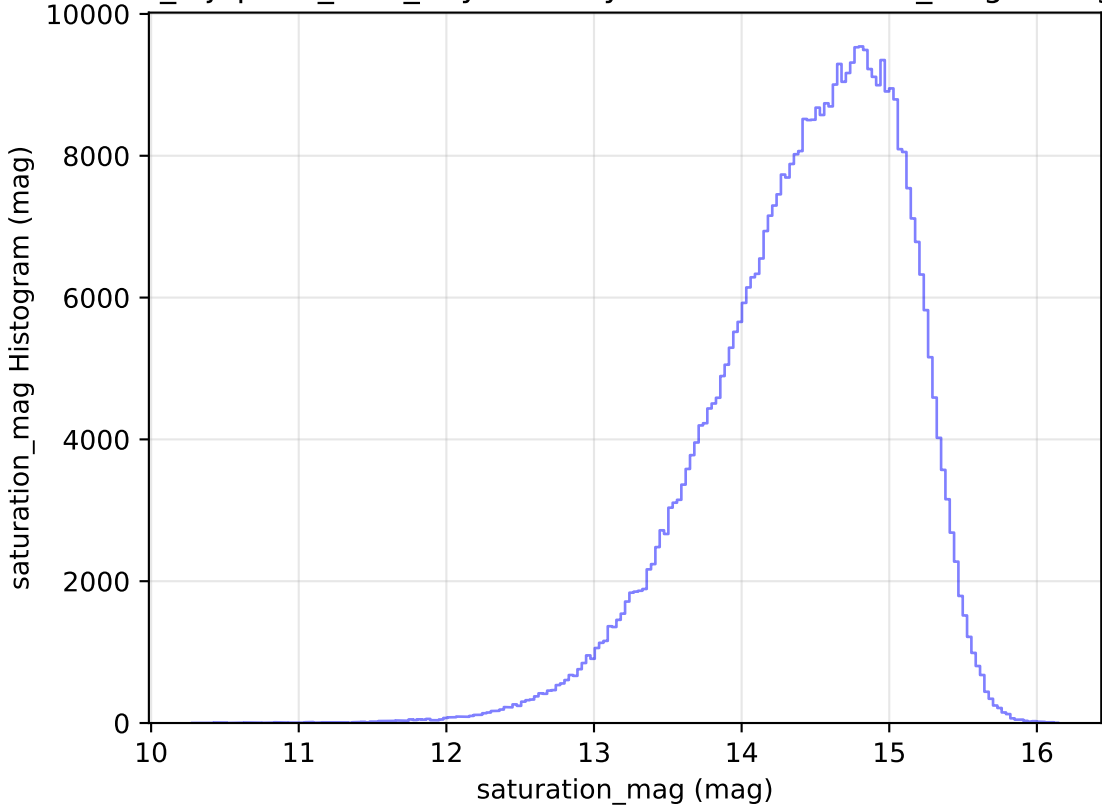
noroll_mjdp180_v3.4_10yrs All sky i band: saturation_mag Histogram
