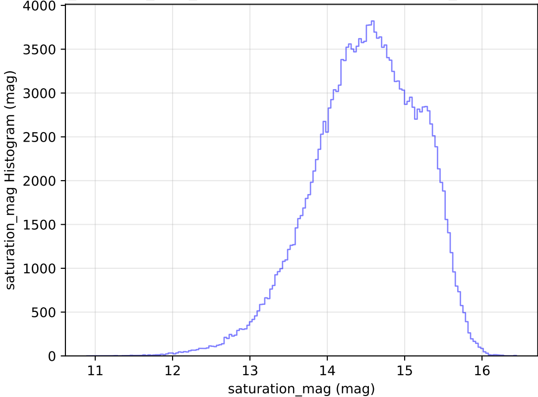
noroll_mjdp180_v3.4_10yrs All sky g band: saturation_mag Histogram
