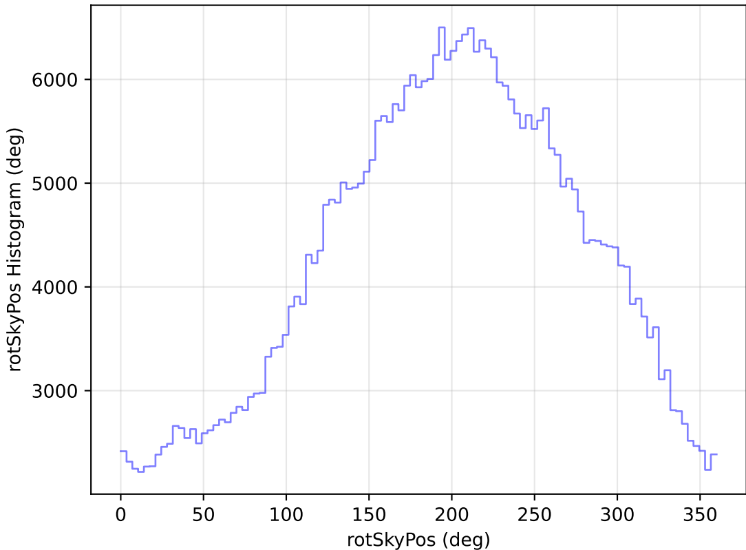
noroll_mjdp180_v3.4_10yrs WFD z band: rotSkyPos Histogram
