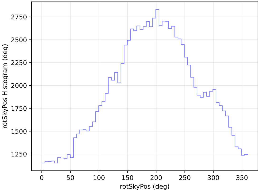
noroll_mjdp180_v3.4_10yrs WFD u band: rotSkyPos Histogram
