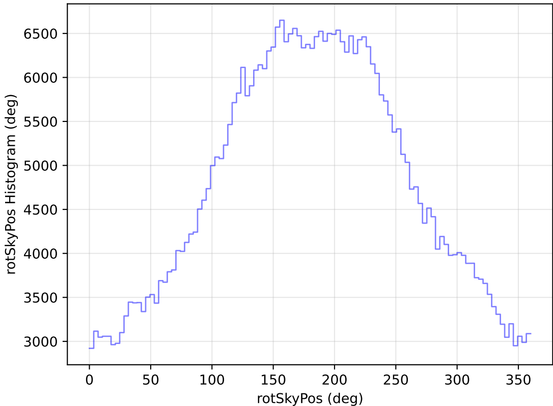
noroll_mjdp180_v3.4_10yrs WFD r band: rotSkyPos Histogram
