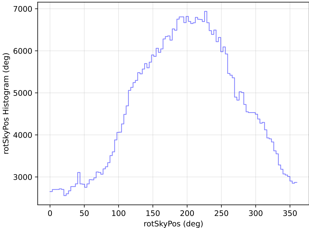
noroll_mjdp180_v3.4_10yrs WFD i band: rotSkyPos Histogram
