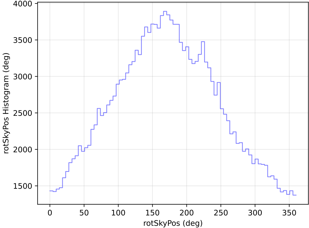
noroll_mjdp180_v3.4_10yrs WFD g band: rotSkyPos Histogram
