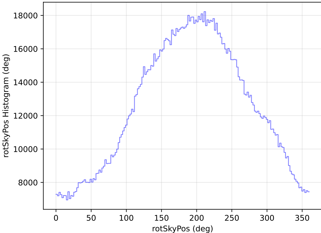
noroll_mjdp180_v3.4_10yrs WFD all bands: rotSkyPos Histogram
